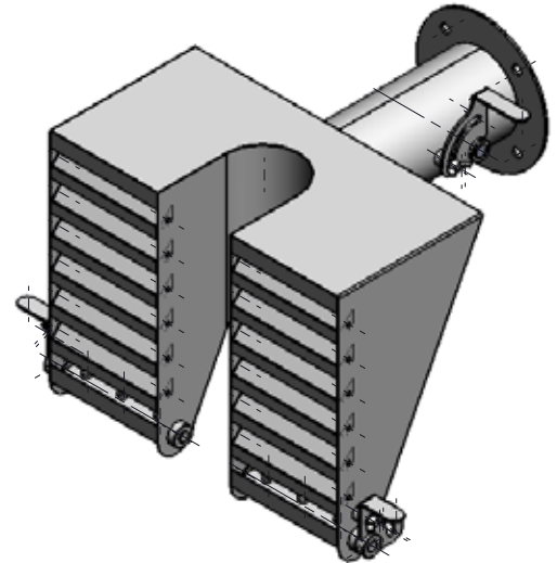
Hood For Weighing Scale Material : SUS Weight : 6.45 Kg. Unit : mm.
